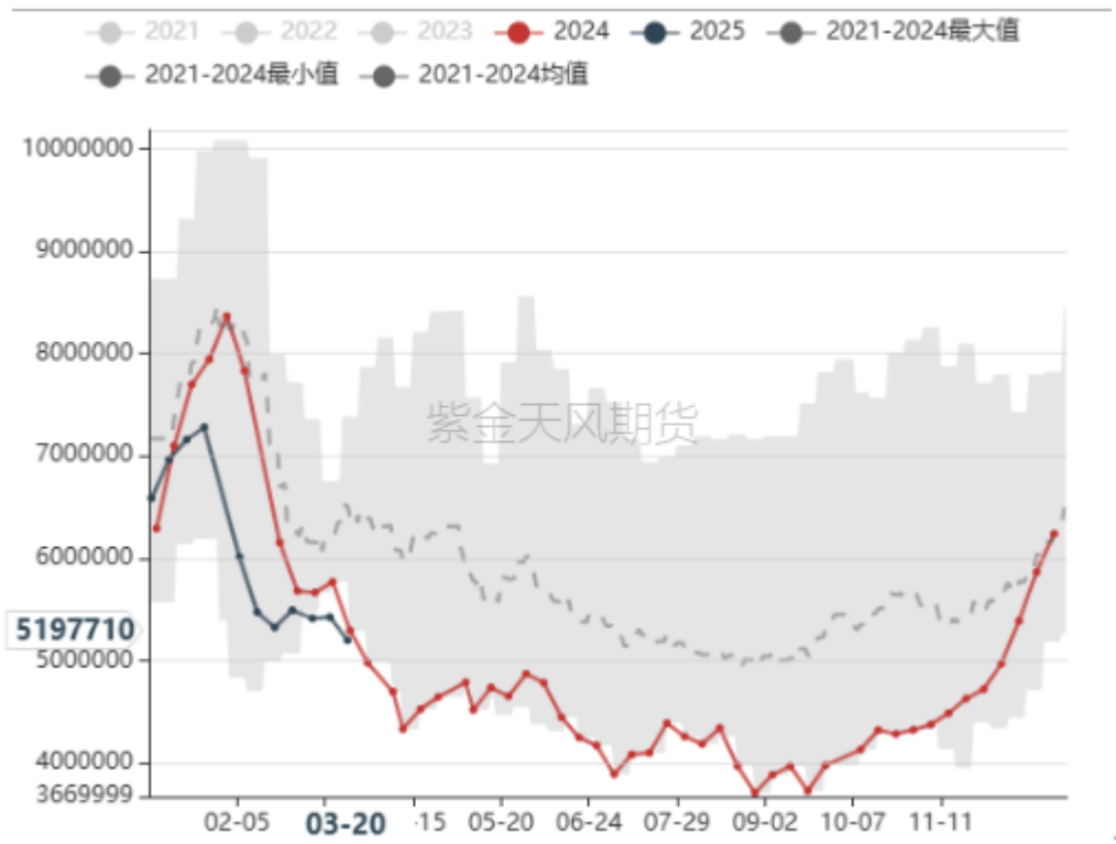
废钢-255家钢厂废钢库存：汇总
